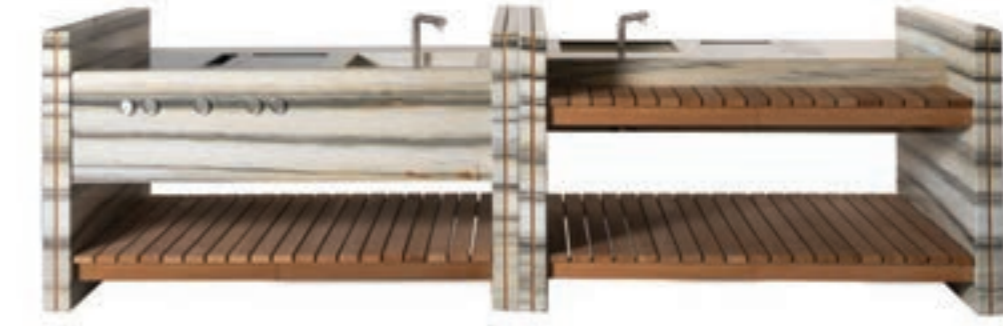
Kitchen Stripes Materials: zebrino, teak, aluminum Weight: 540 kg Dimensions: L180cm - P122cm - H90cm
